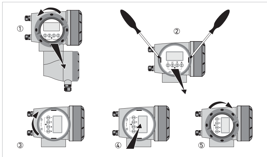
Figure 3-17: Turning the display of the field housing version
