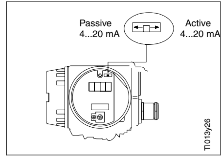
Location of the current output passive/active configuration switch on the terminal connection printed circuit board
