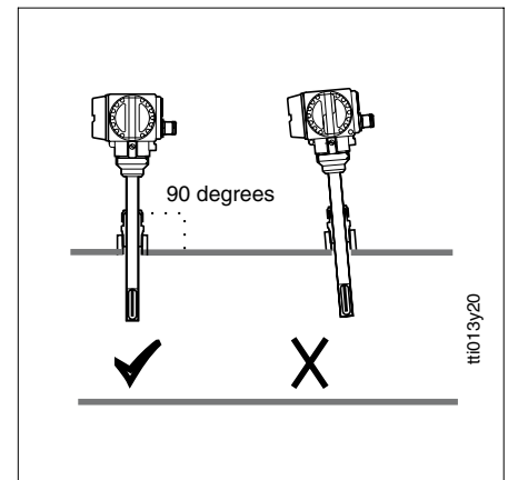
Vertical alignment
