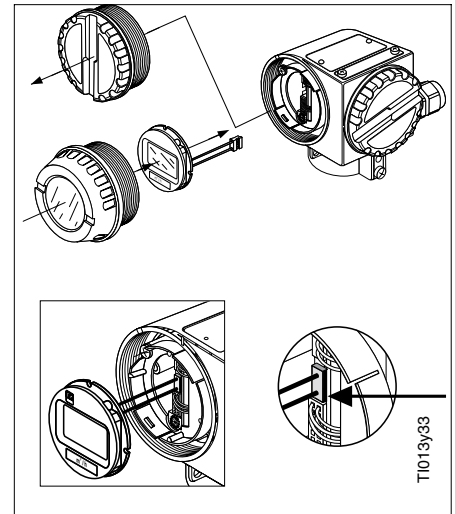
Mounting/ removing the local display module Location of the pulse/current output configuration switches in the main electronics compartment after
