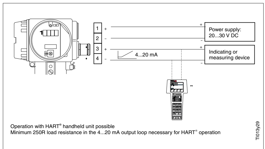
Active current output wiring
