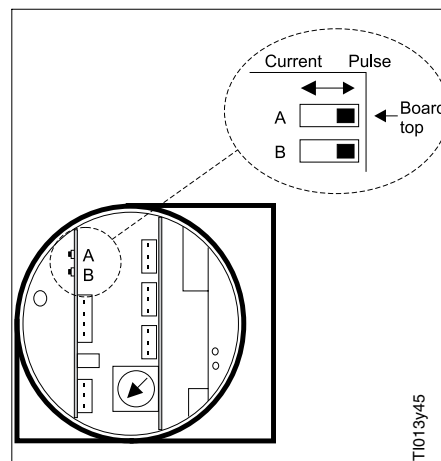
Location of the pulse/current selection switches after the display and display bezel have been removed - Remote Electronics version only
