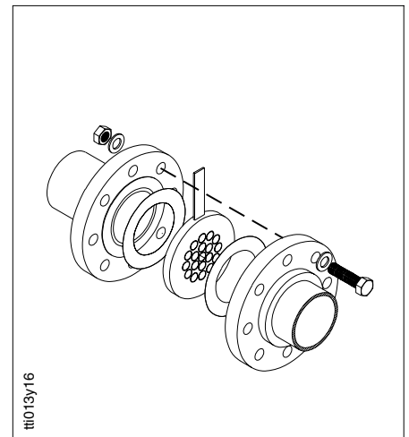
AZT532 and AZT534 flowconditioner mounting arrangement
