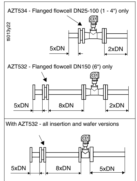
Using the flow conditioner
