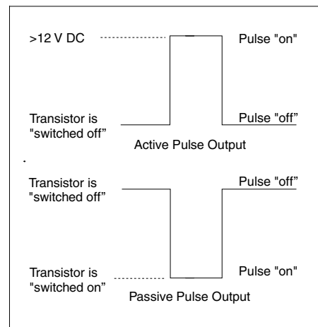
Active and passive pulse output waveforms
