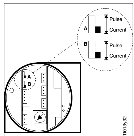
Location of the pulse/current selection switches after the display and display bezel have been removed - Compact sensor version only
