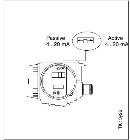
Location of passive/active configuration switch on the terminal connection printed circuit board
