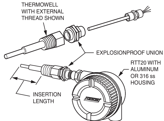
Figure 3. RTT20 with Integral Sensor with Thermowell
