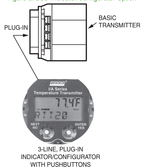
Figure 2. LCD Indicator/Configurator Option
