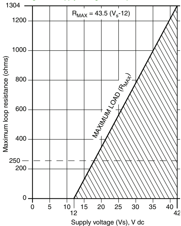
Figure 4. Supply Voltage vs. Output Load
