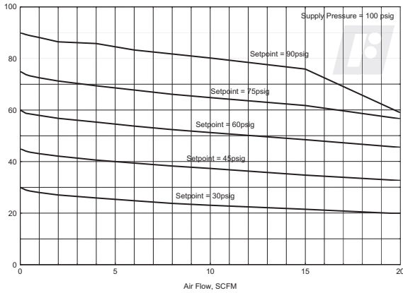
Flow Characteristics Fairchild Model 65952
