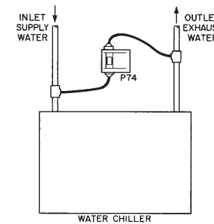
Figure 3: Typical proof of flow hookup.
