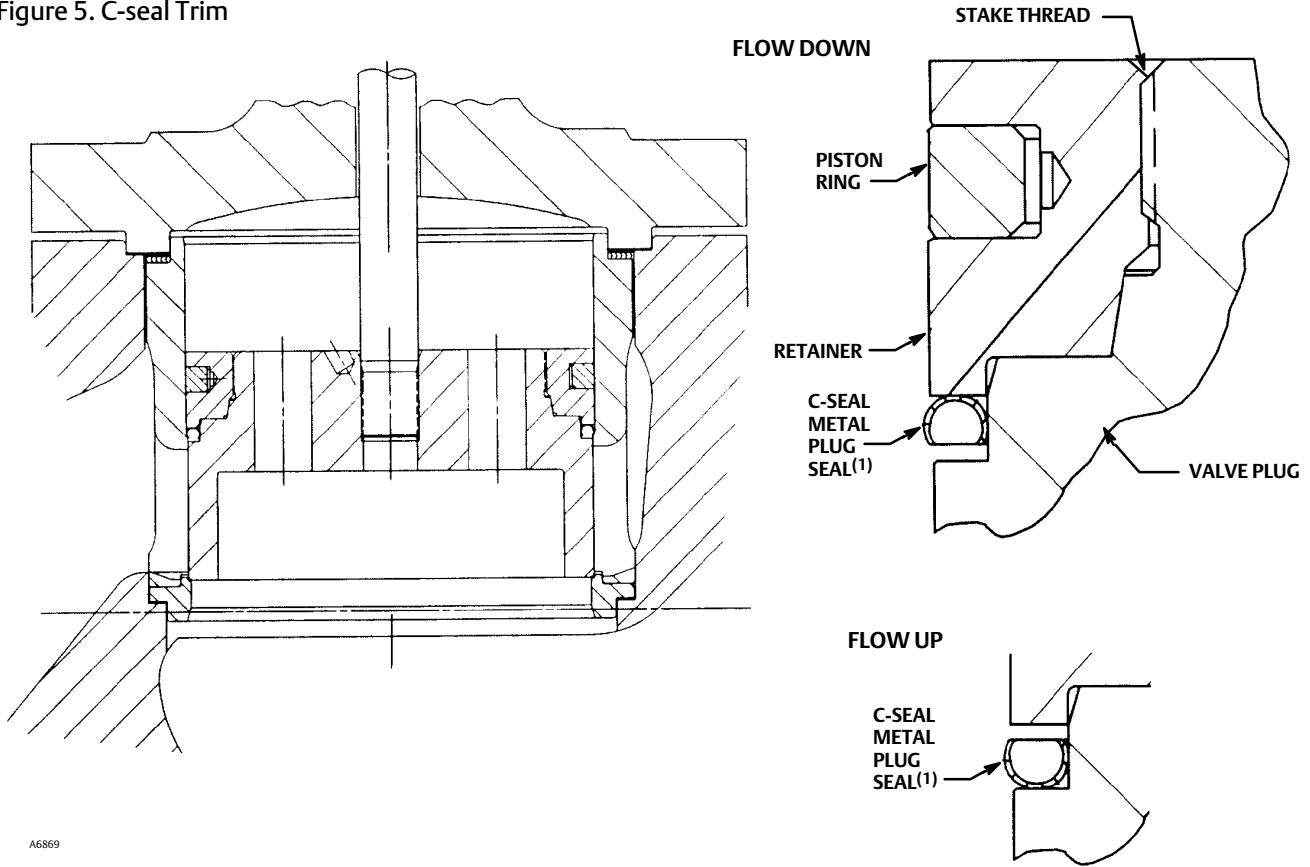
Figure 5. C-seal Trim
