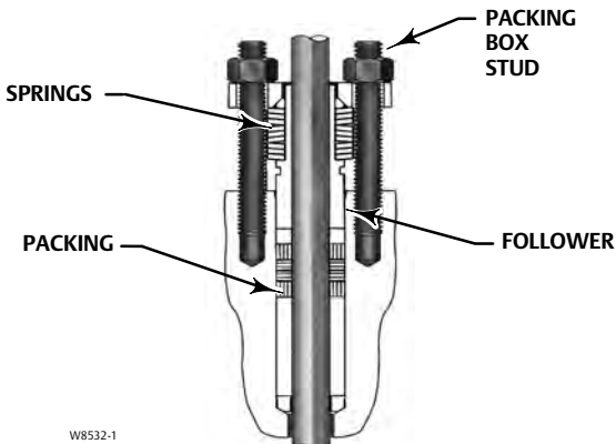
TYPICAL ENVIRO-SEAL PACKING SYSTEM WITH GRAPHITE ULF PACKING
