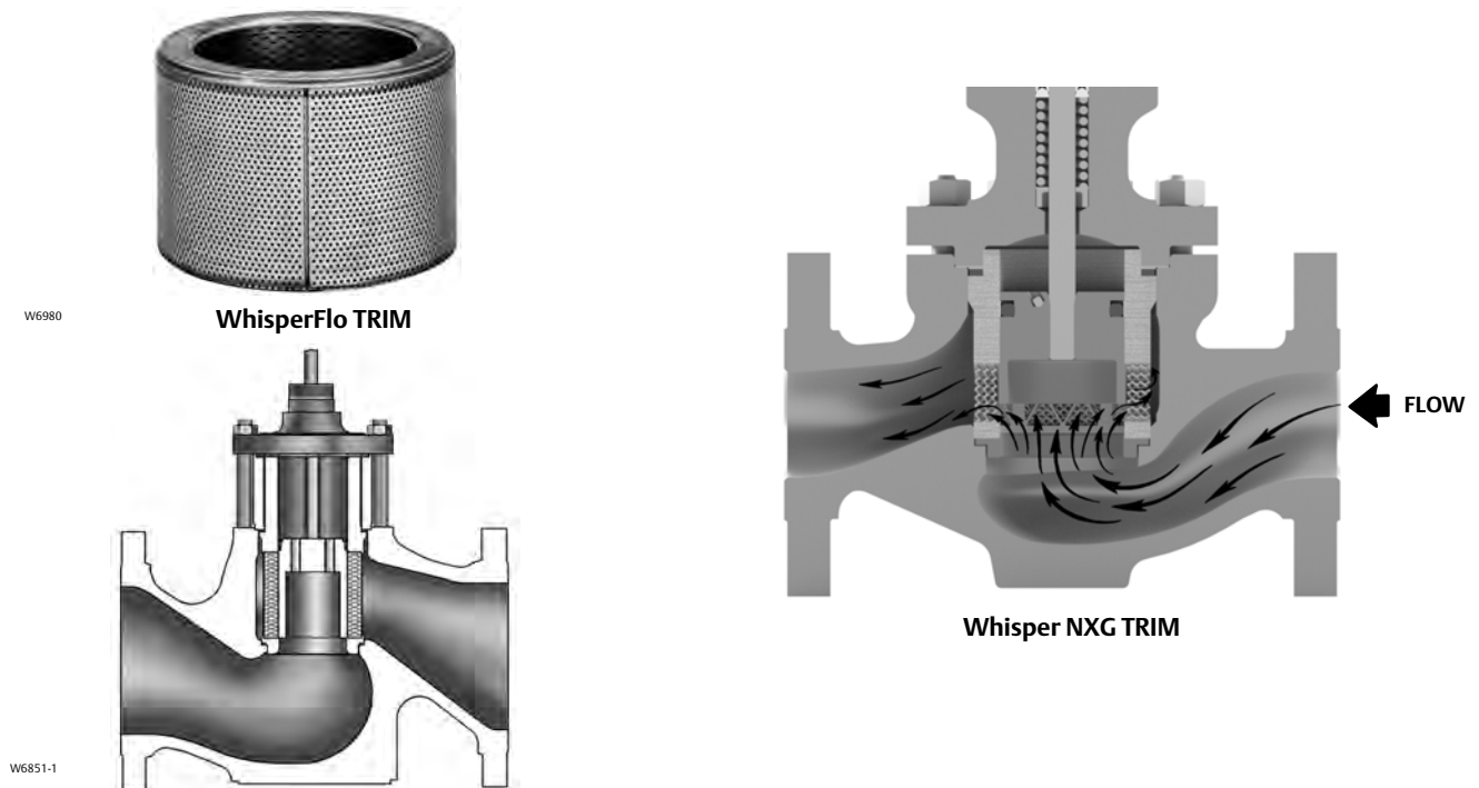
Figure 4. Typical Valve with WhisperFlo Aerodynamic or Whisper NXG Trim
