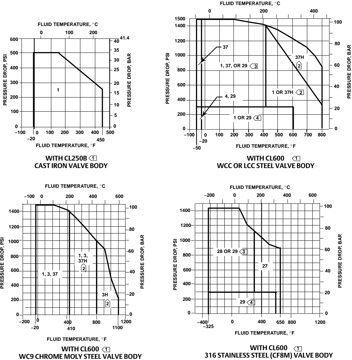
Figure 9. Typical Trim Used for All Valves Except with Whisper Trim III Cage, Whisper NXG Trim, and WhisperFlo Cage
