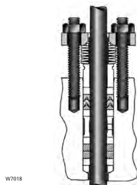
TYPICAL ENVIRO-SEAL PACKING SYSTEM WITH DUPLEX PACKING
