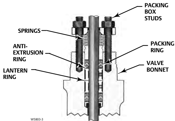
TYPICAL ENVIRO-SEAL PACKING SYSTEM WITH PTFE PACKING
