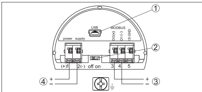
Fig. 27: Terminal compartment
