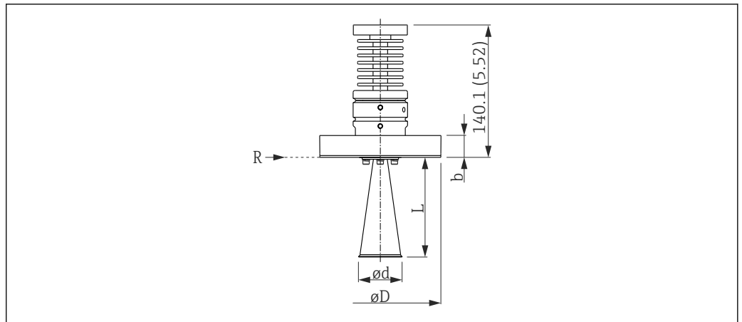
26 FMR51: Version T < 450\text{ °C} (842 °F); dimensions: mm (in)
