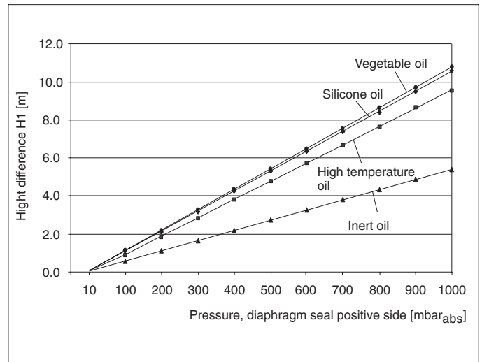
Diagram of maximum installation height above the lower diaphragm seal for vacuum applications dependent on the pressure at the diaphragm seal on the positive side.
