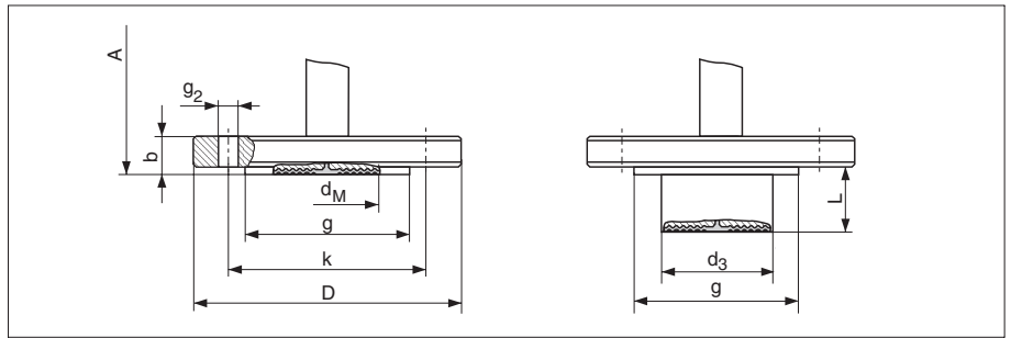
Diaphragm seal flange, connection dimensions according to EN 1092-1/DIN 2527, material: AISI 316L (1.4435)
