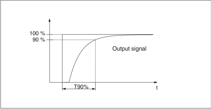
Presentation of the response time (T90%)
