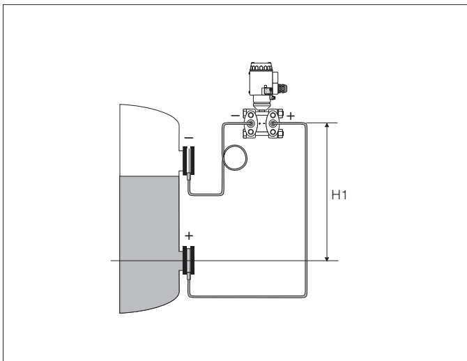
Installation above the lower diaphragm seal
